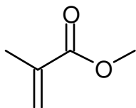
methyl methacrylate
